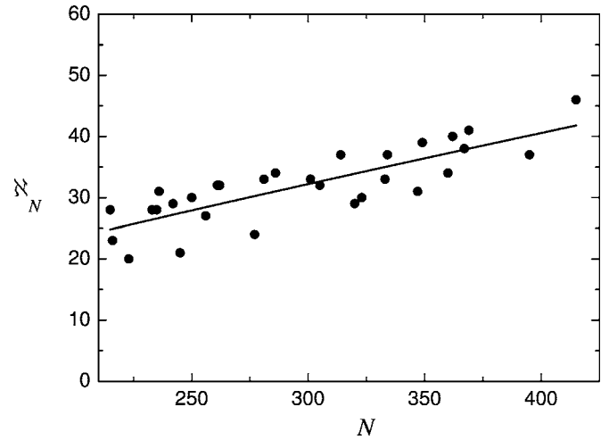
FIG. 6. The number of nodal domains \aleph_N (full circles) for the chaotic half-circular microwave ray-splitting rough billiard. Full line shows the least squares fit \aleph_N = a_1 N + b_1 \sqrt{N} to the experimental data (see text), where a_1 = 0.063 \pm 0.023 , b_1 = 0.77 \pm 0.40 . The prediction of the theory of Bogomolny and Schmit [1] a_1 = 0.062 .
