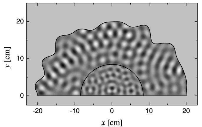
FIG. 3. The reconstructed wave function \Psi_{415}(r, \theta) of the chaotic half-circular microwave rough billiard. The amplitudes have been converted into a gray scale with white corresponding to large positive and black corresponding to large negative values, respectively. Dimensions of the billiard are given in cm. The position of the half-circular Teflon insert of radius R_d = 8.465 cm is marked with a solid line.
