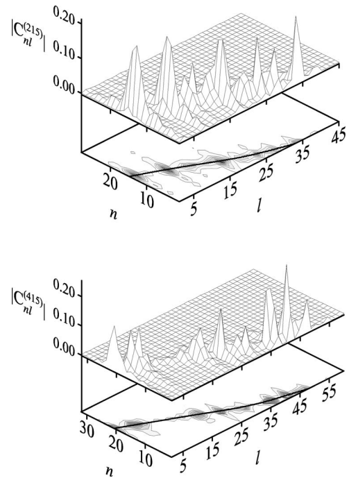
FIG. 4. Structure of the energy surface in the regime of Shnirelman ergodicity. Here we show the moduli of amplitudes |C_{nl}^{(N)}| for the wave functions (a) N=215 , (b) N=415 . The wave functions are delocalized in the n, l basis. Full lines show the energy surface (see text).
