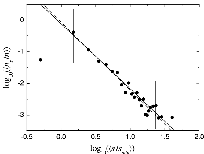
FIG. 8. Distribution of nodal domain areas. Full line shows the prediction of percolation theory \log_{10}(\langle n_s/n \rangle) = -187/91 \log_{10}(\langle s/s_{min} \rangle) . The least squares fit \log_{10}(\langle n_s/n \rangle) = a_2 - \tau \log_{10}(\langle s/s_{min} \rangle) of the experimental results lying within the vertical lines yields the scaling exponent \tau = 2.14 \pm 0.12 and a_2 = -0.06 \pm 0.12 . The result of the fit is shown by the dashed line.
