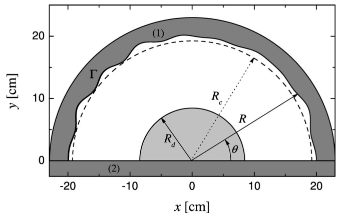
FIG. 1. Sketch of the chaotic half-circular microwave ray-splitting rough billiard which consists a half-circular Teflon insert of radius R_d = 8.465 cm. Dimensions are given in cm. The cavity side-walls are marked by 1 and 2 (see text). Squared wave functions |\Psi_N(R_c, \theta)|^2 were evaluated on a half-circle of fixed radius R_c = 19.25 cm. The billiard's rough boundary is marked by \Gamma .
