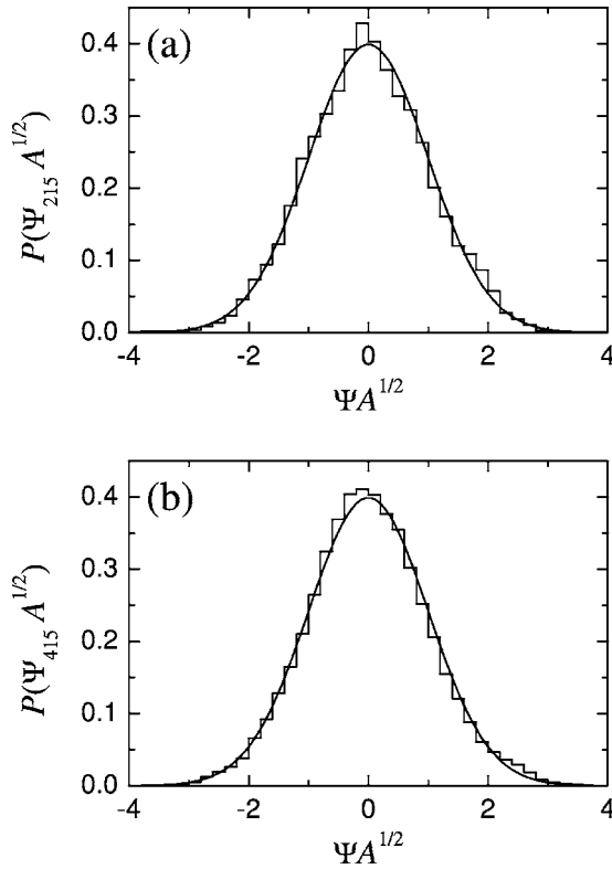
FIG. 5. (a) The amplitude distribution P(\Psi_N A^{1/2}) for the wave function N=215 . (b) The distribution P(\Psi_N A^{1/2}) for the wave function N=415 . The amplitude distributions were constructed as histograms with bin equal to 0.2. The width of the distribution P(\Psi) was rescaled to unity by multiplying normalized to unity wave function by the factor A^{1/2} , where A denotes the billiard's area. Full lines show standard normalized Gaussian prediction P_0(\Psi A^{1/2}) = (1/\sqrt{2\pi})e^{-\Psi^2 A/2} .
