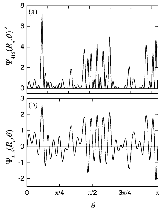
FIG. 2. (a) Squared wave function |\Psi_{415}(R_c, \theta)|^2 (in arbitrary units) measured on a half-circle with radius R_c = 19.25 cm ( \nu_{415} \approx 12.98 GHz). (b) The ‘‘trial wave function’’ \Psi_{415}(R_c, \theta) (in arbitrary units) with the correctly assigned signs, which was used in the reconstruction of the wave function \Psi_{415}(r, \theta) of the billiard (see Fig. 3).
